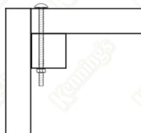
CORNER INSTALLATION
